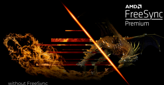
without FreeSync
