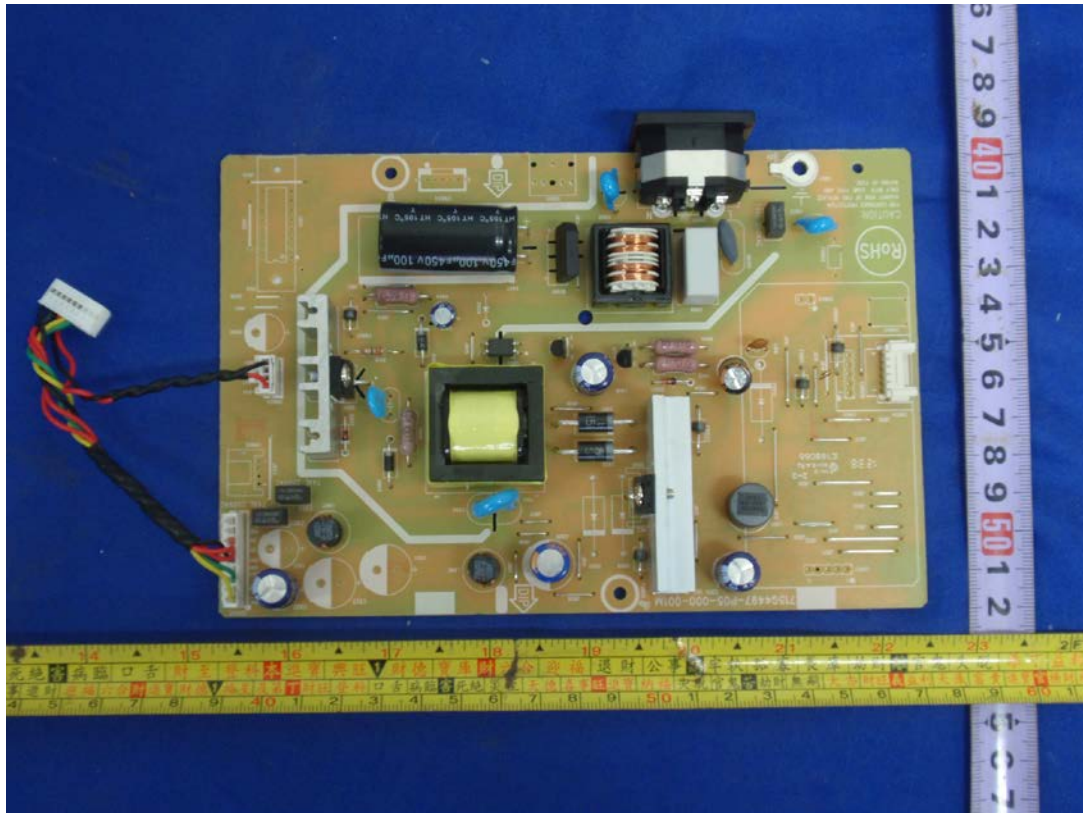
Figure 29. Power board 715G4497 type C
