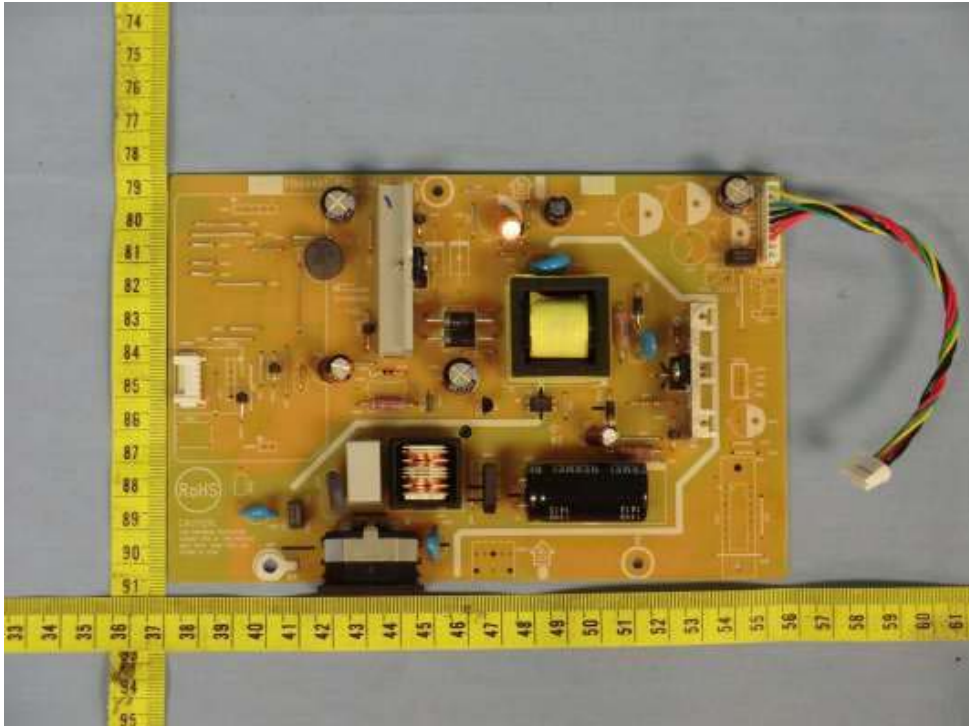
Figure 25. Power board 715G4497 type A
