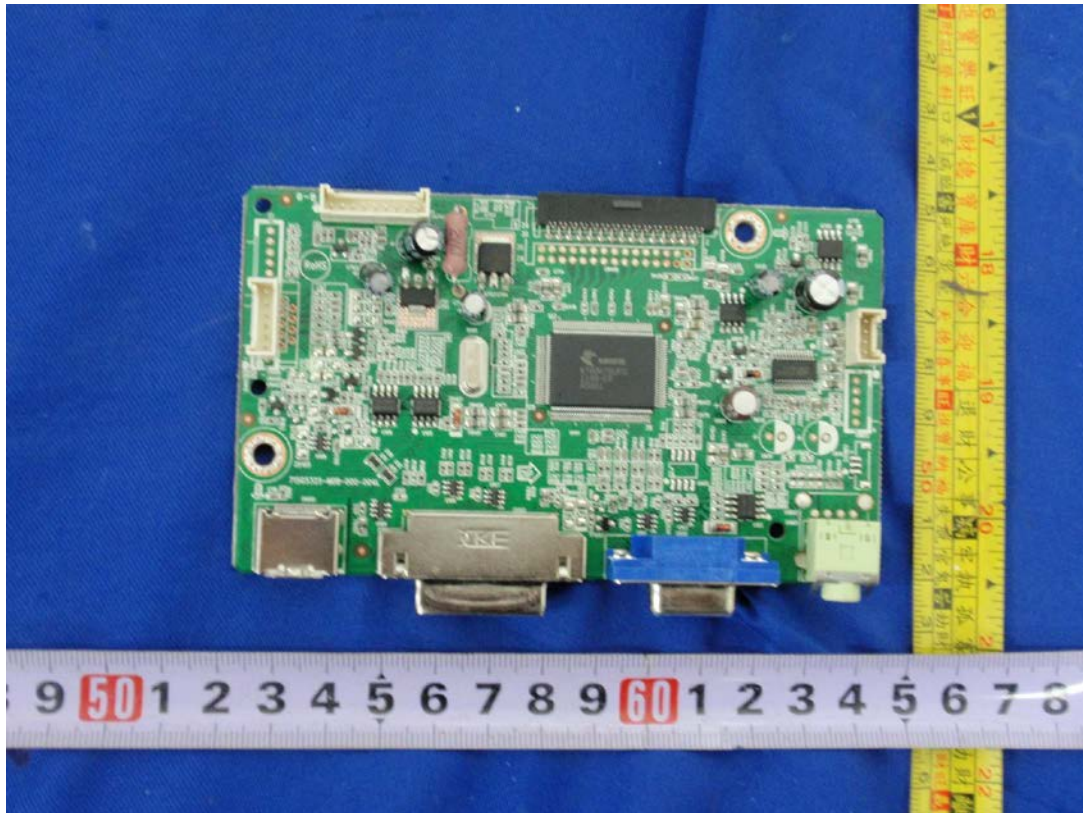
Figure 35. Main board 715G5325
