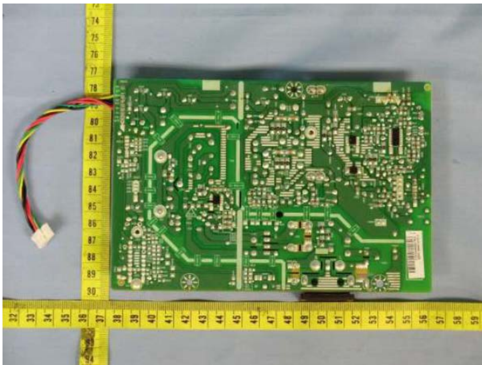
Figure 26. Power board 715G4497 type A
