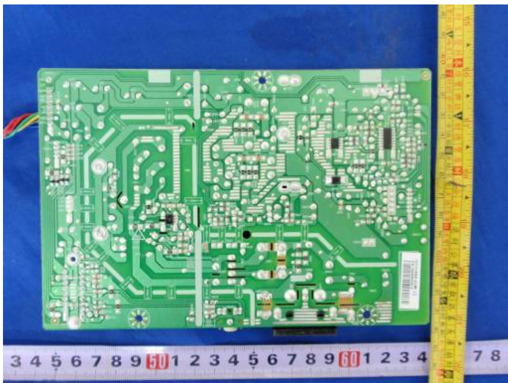
Figure 28. Power board 715G4497 type B
