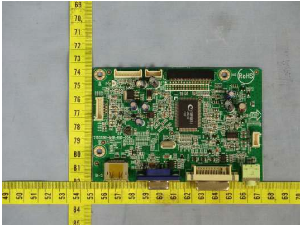
Figure 31. Main board 715G5281
