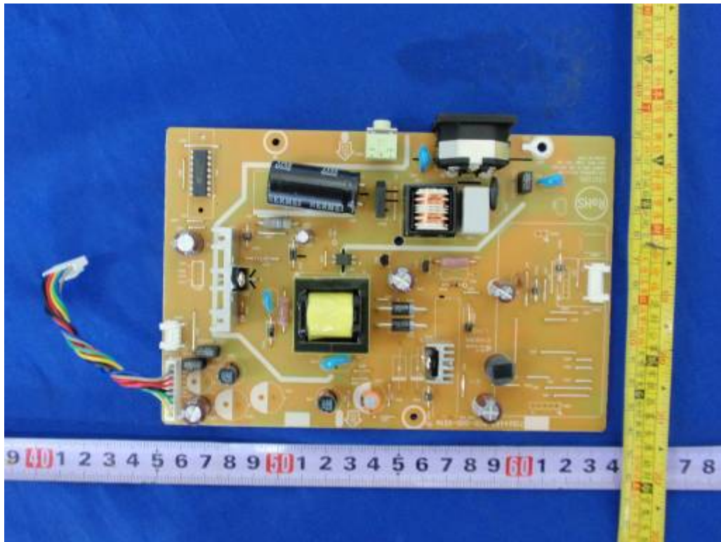
Figure 27. Power board 715G4497 type B
