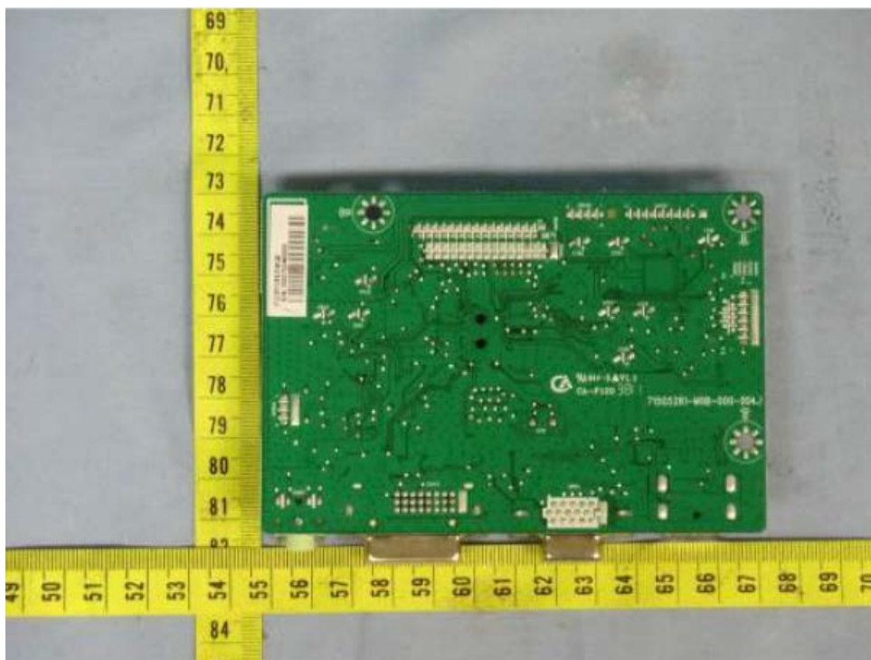
Figure 32. Main board 715G5281
