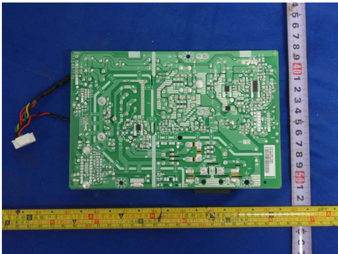
Figure 30. Power board 715G4497 type C
