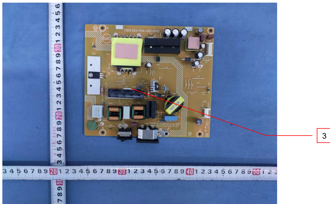
Photo 4 - Power board (TPV / 715GF253)
