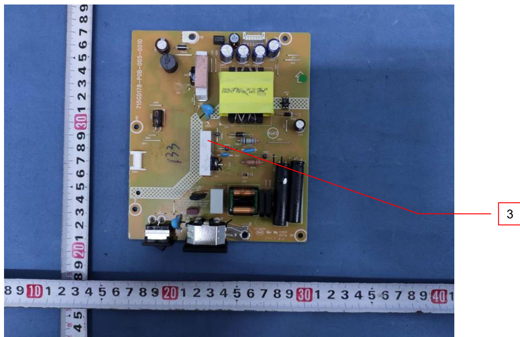
Photo 4 - Power board (TPV / 715GD178)
