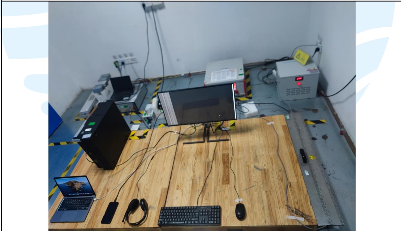
Fast Transients, Common mode (Wired network ports) Test Setup
