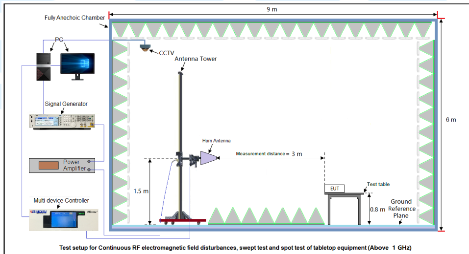
Figure 2. Above 1 GHz
