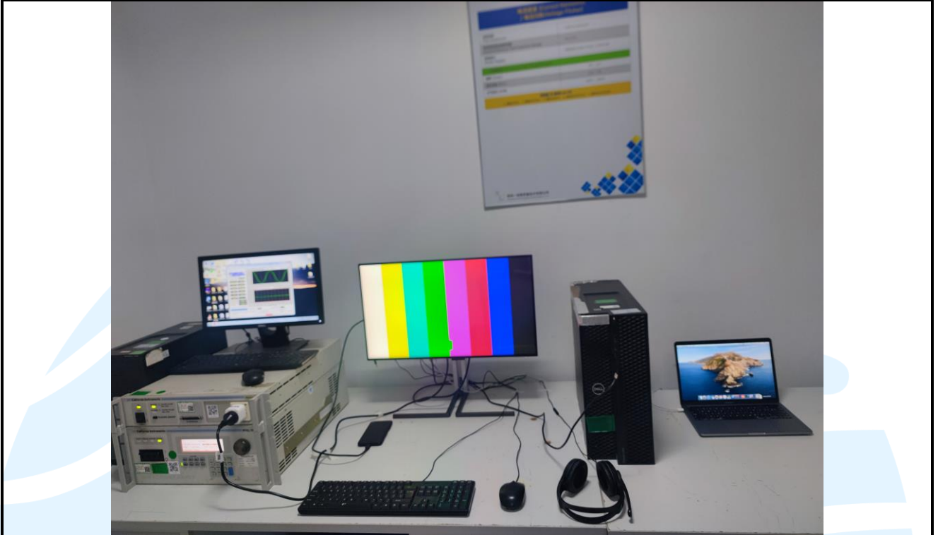
Harmonic & Flicker Test Setup
