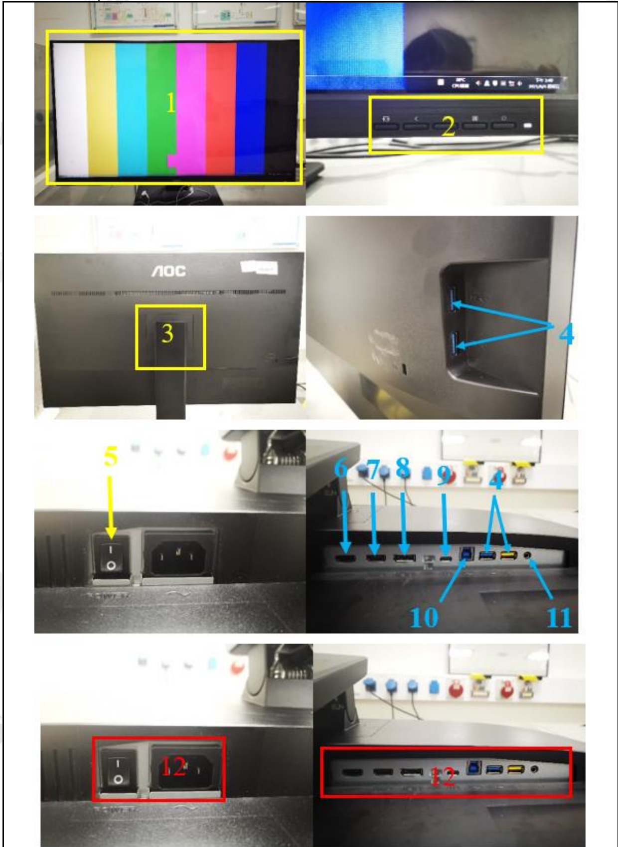
Photo of ESD point on EUT
