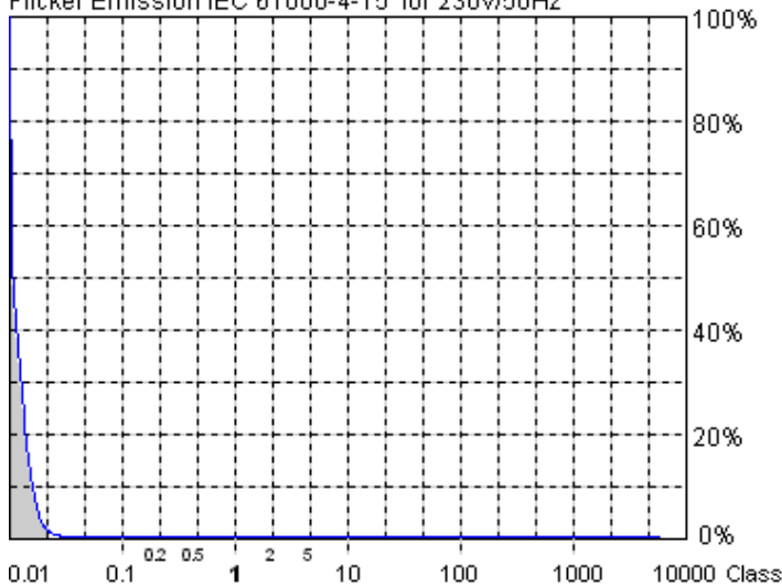
Flicker Emission IEC 61000-4-15 for 230V/50Hz
