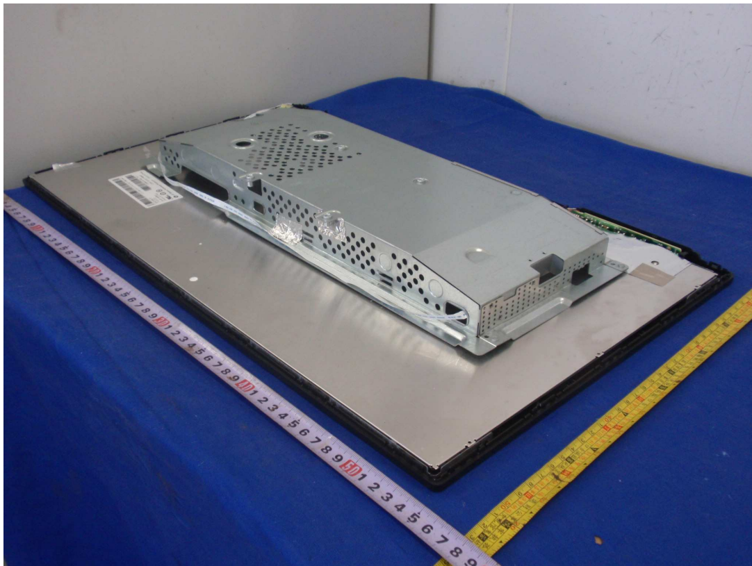
Figure 16 Metal enclosure type B
