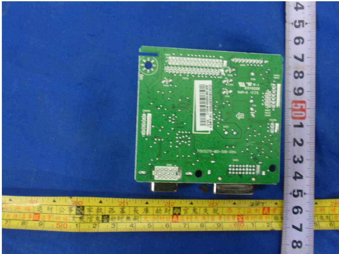
Figure 21 Main board
