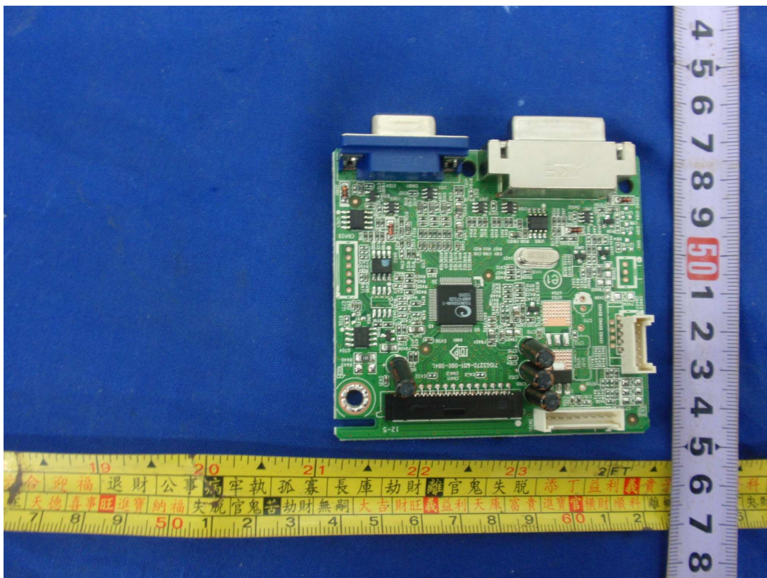
Figure 20 Main board
