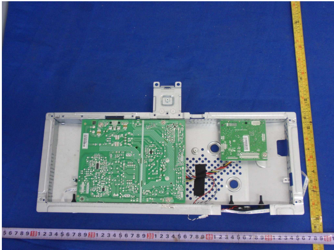
Figure 13 Metal enclosure type A
