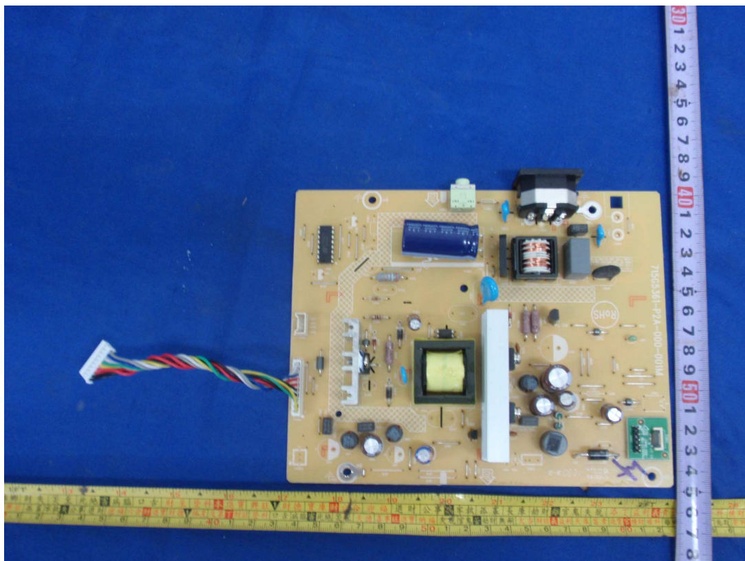
Figure 18 Power board
