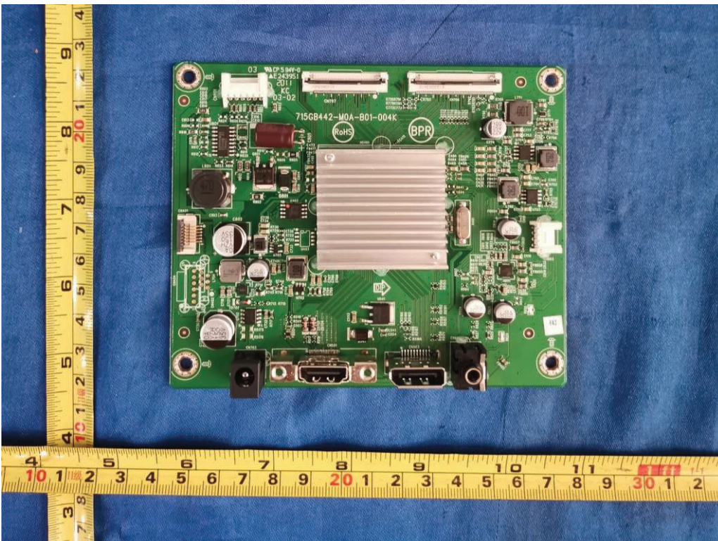
Figure 22. Main board 715GB442
