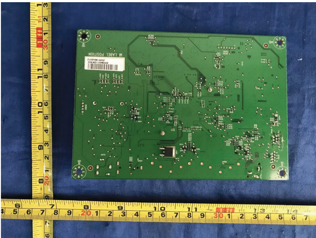
Figure 16. Main board 715G9500
