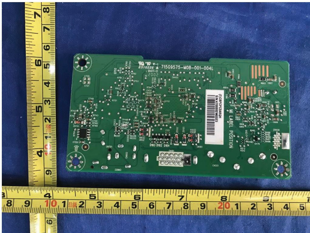
Figure 8. Main board 715G9575
