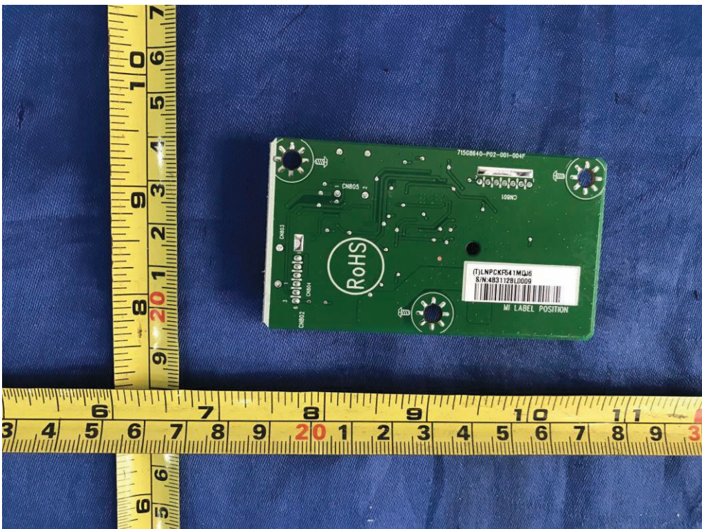
Figure 18. DC converter 715G8640
