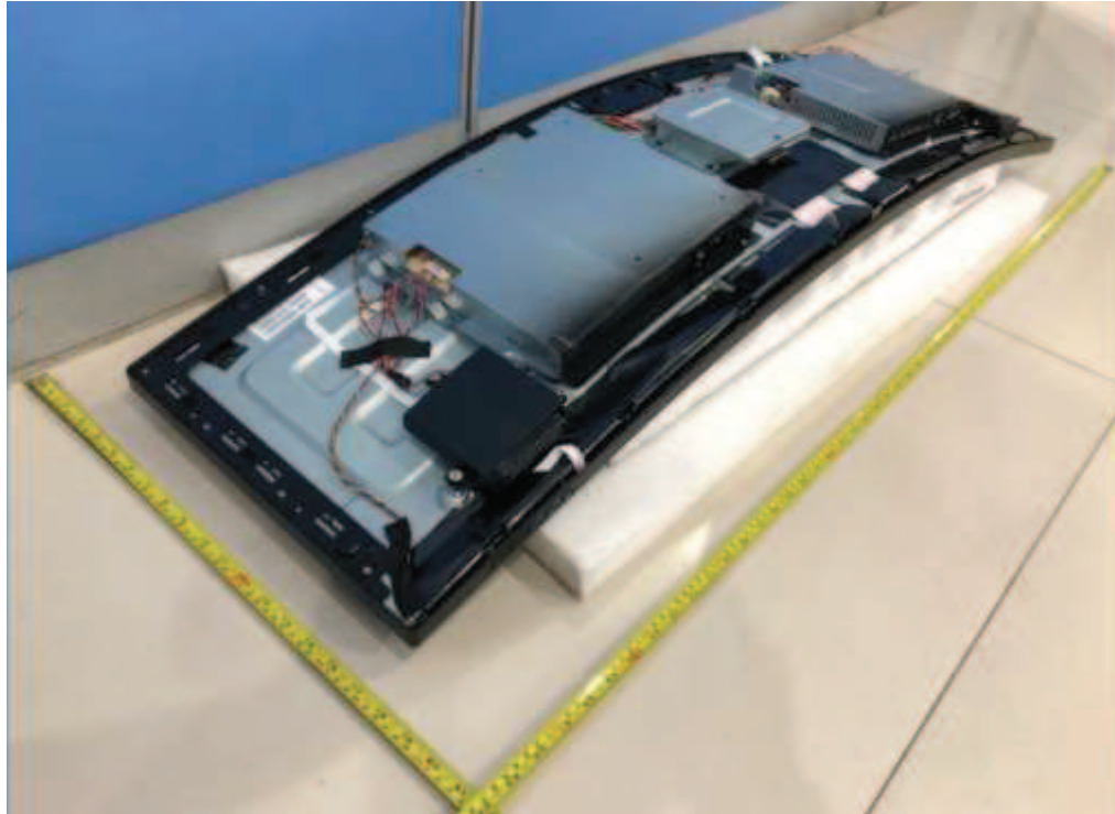
Figure 7. Internal view
