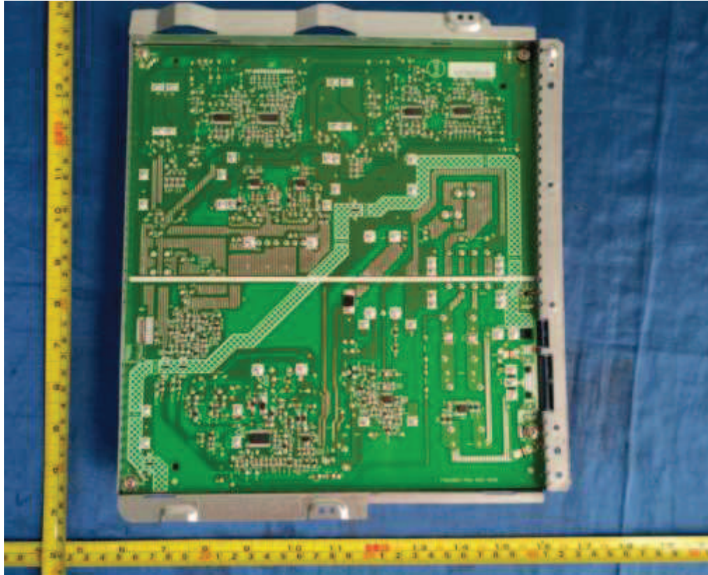
Figure 9. Internal view
