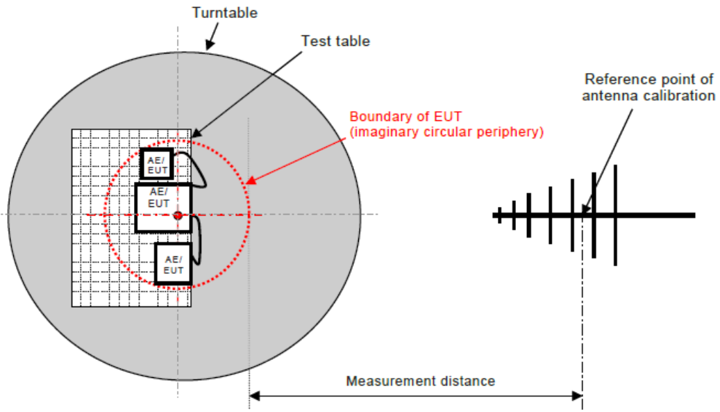
Figure C.1 – Measurement distance
