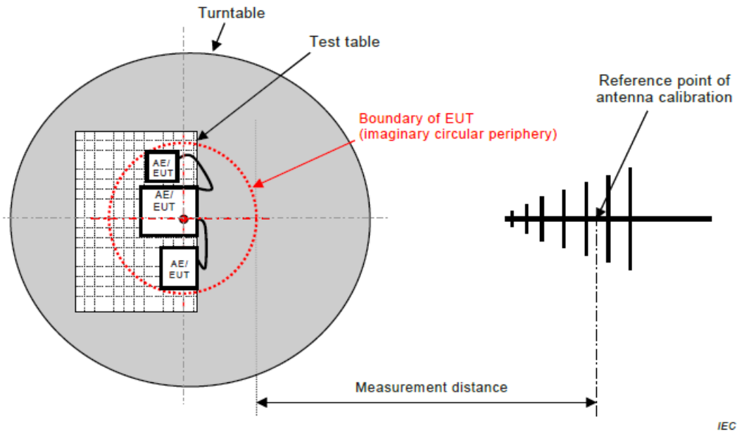
Figure C.1 – Measurement distance
