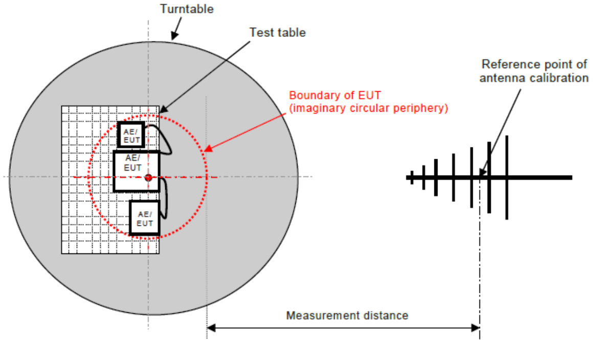
Figure C.1 – Measurement distance
