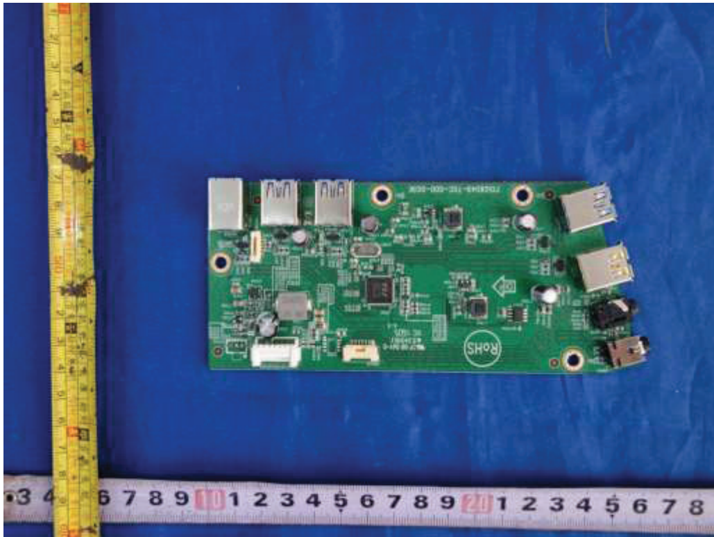
Figure 15. USB board 715G8049
