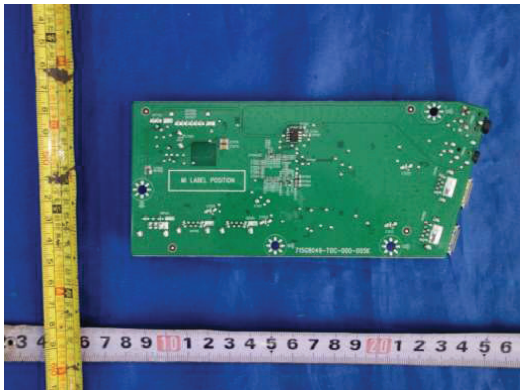
Figure 16. USB board 715G8049
