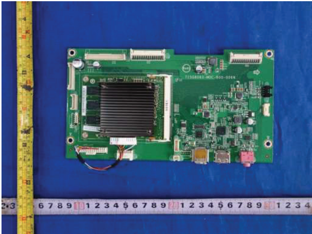
Figure 13. Main board 715G8083
