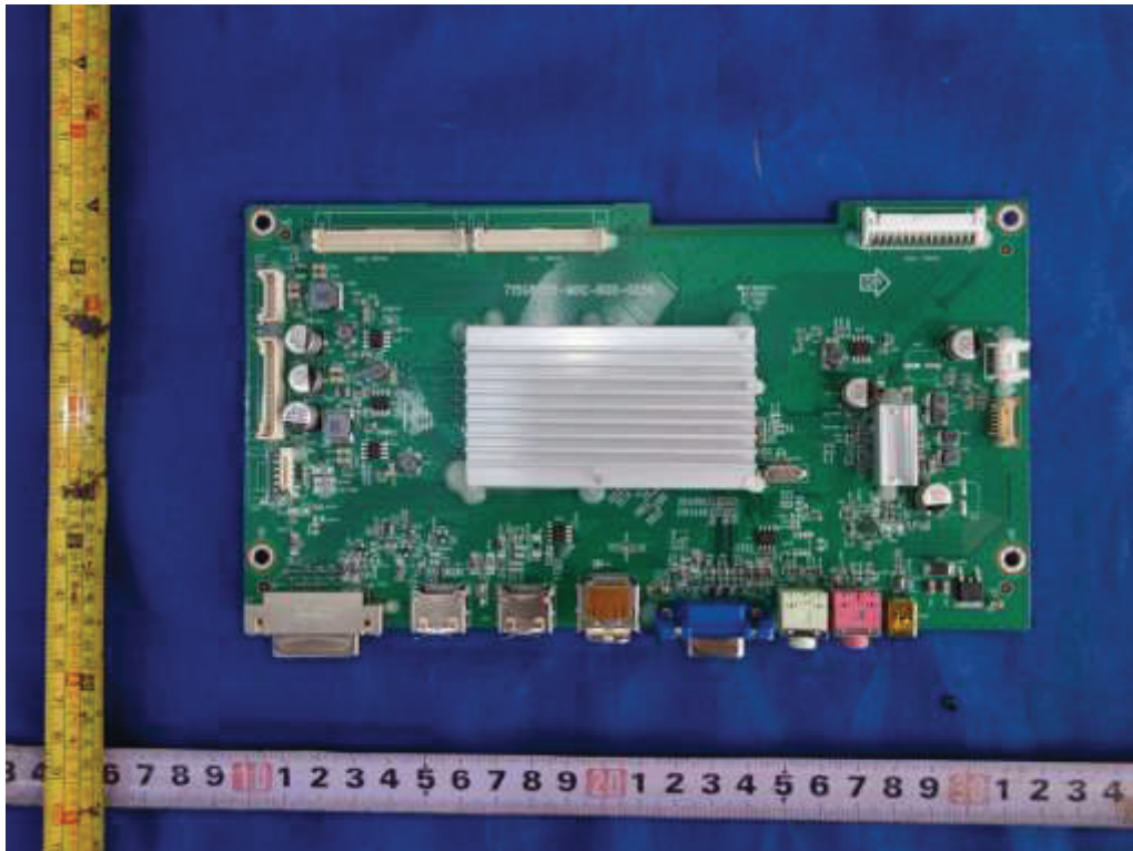
Figure 11. Main board 715G8055
