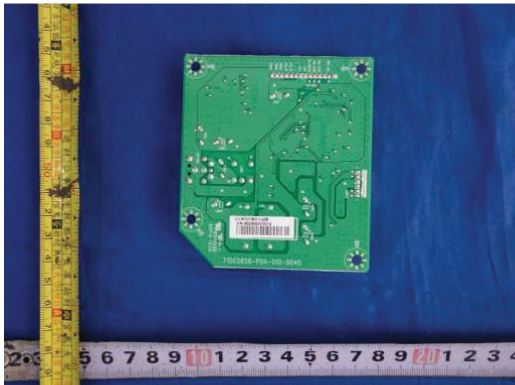
Figure 10. DC/DC converter board 715G5858
