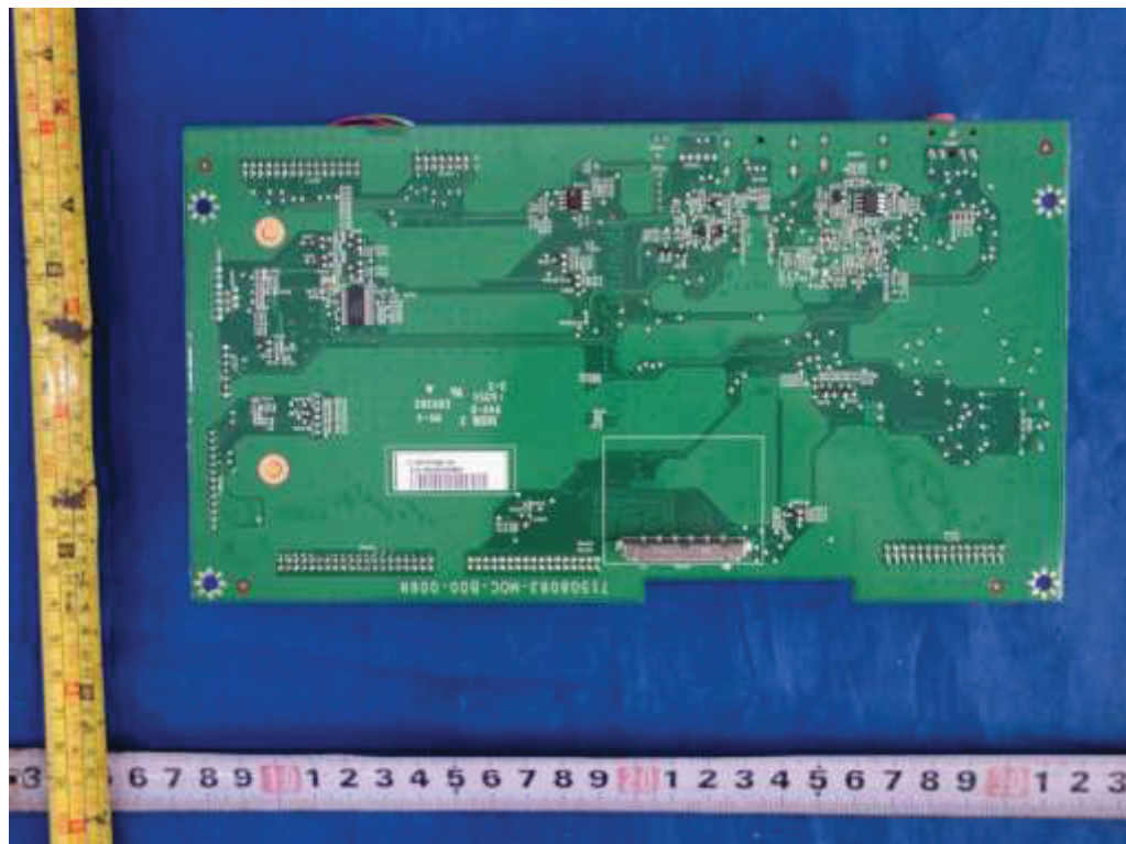
Figure 14. Main board 715G8083
