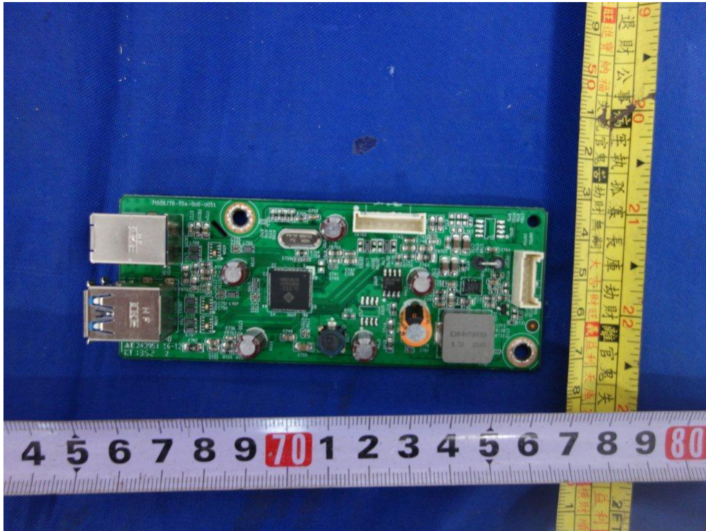
Figure 13. External USB board 715G6770
