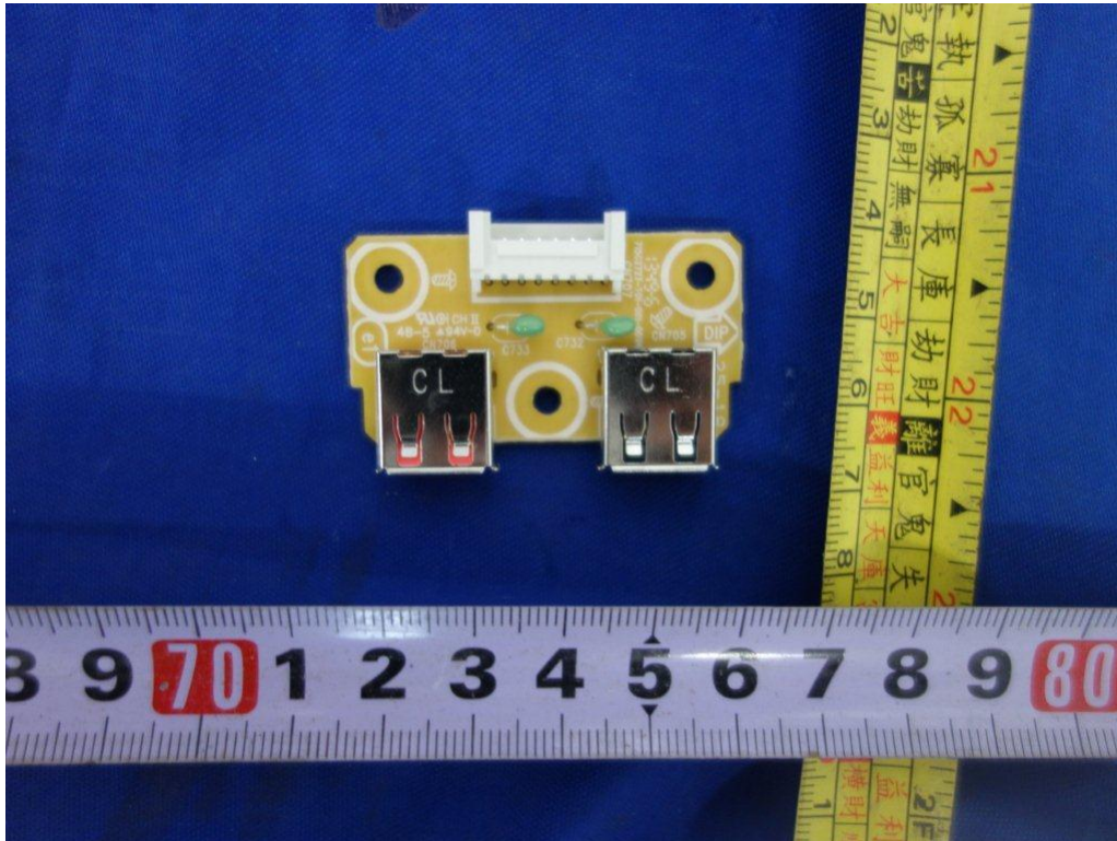
Figure 15. External USB interface board 715G3771
