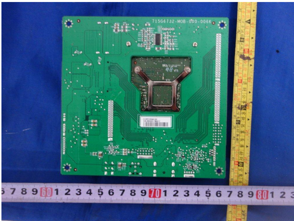
Figure 12. Main board 715G6732
