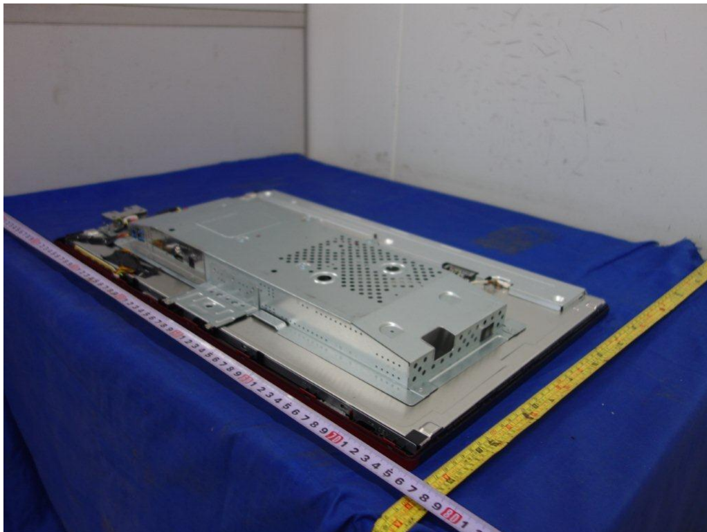
Figure 8. Internal view for metal enclosure
