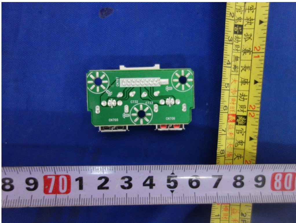
Figure 16. External USB interface board 715G3771
