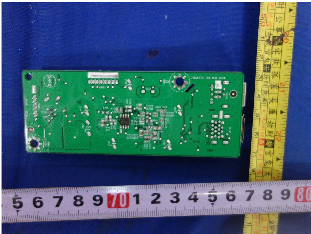
Figure 14. External USB board 715G6770
