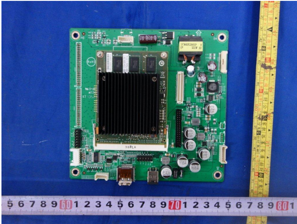
Figure 11. Main board 715G6732
