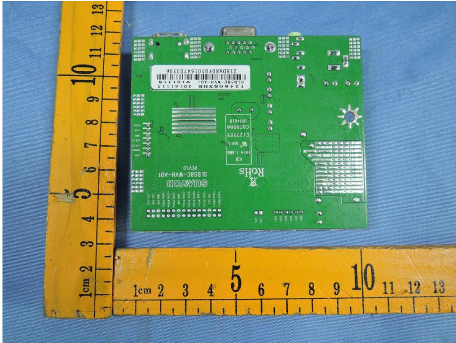
Figure 5. Interface board
