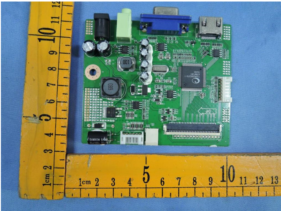
Figure 4. Interface board
