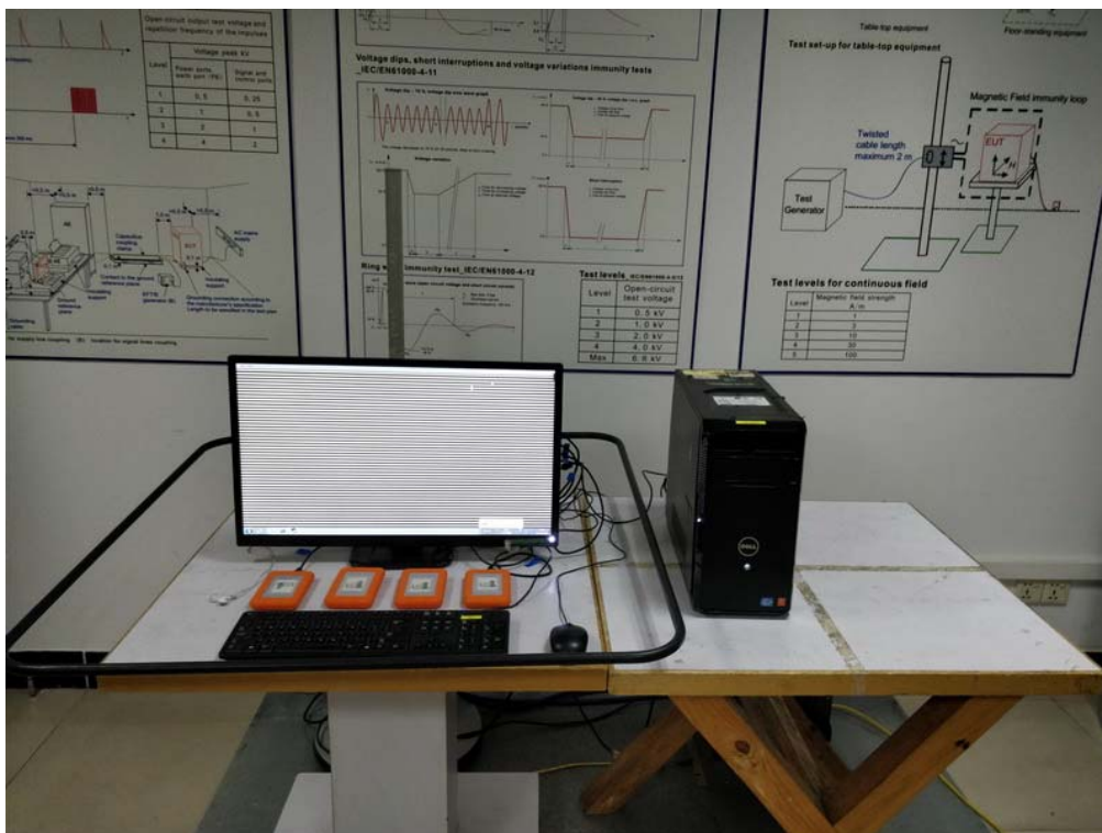
Power frequency magnetic field immunity
