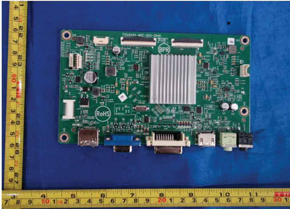
Figure 17. Main board 715G9484
