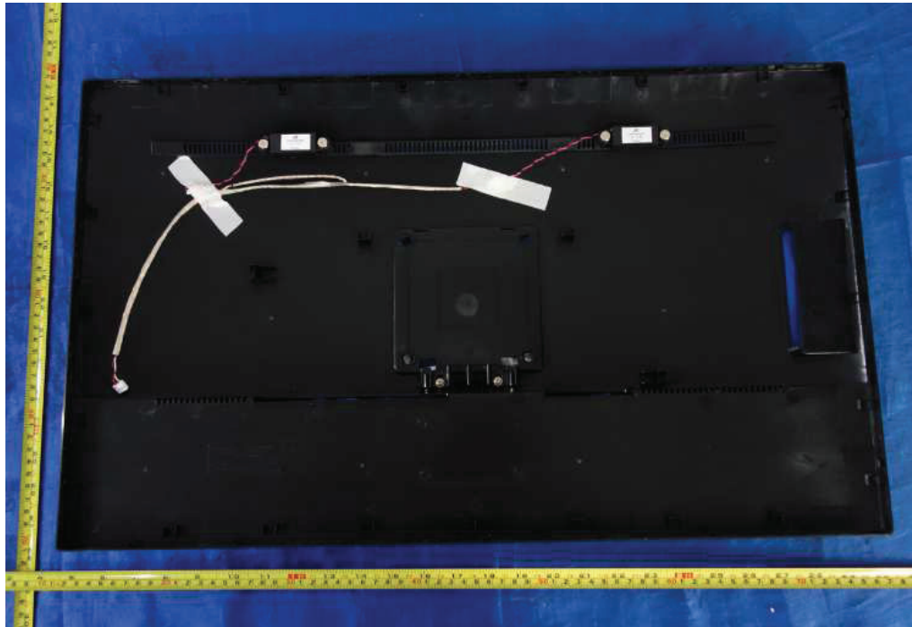
Figure 5. Internal view of plastic enclosure
