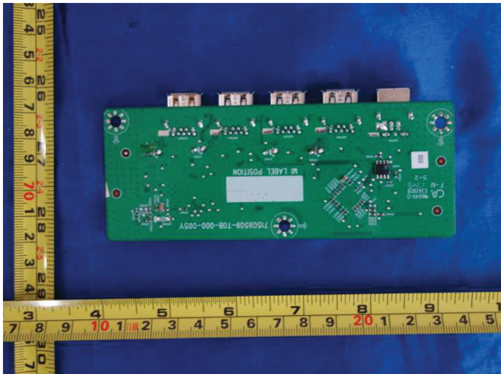
Figure 20. USB board 715G9509
