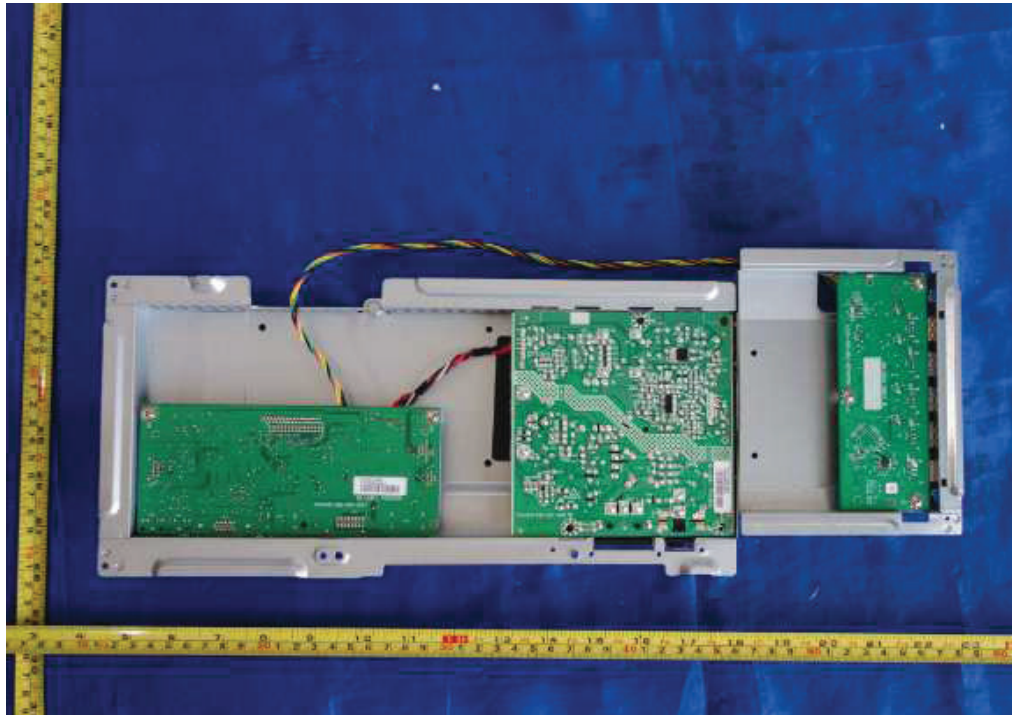
Figure 11. Internal view of metal enclosure
