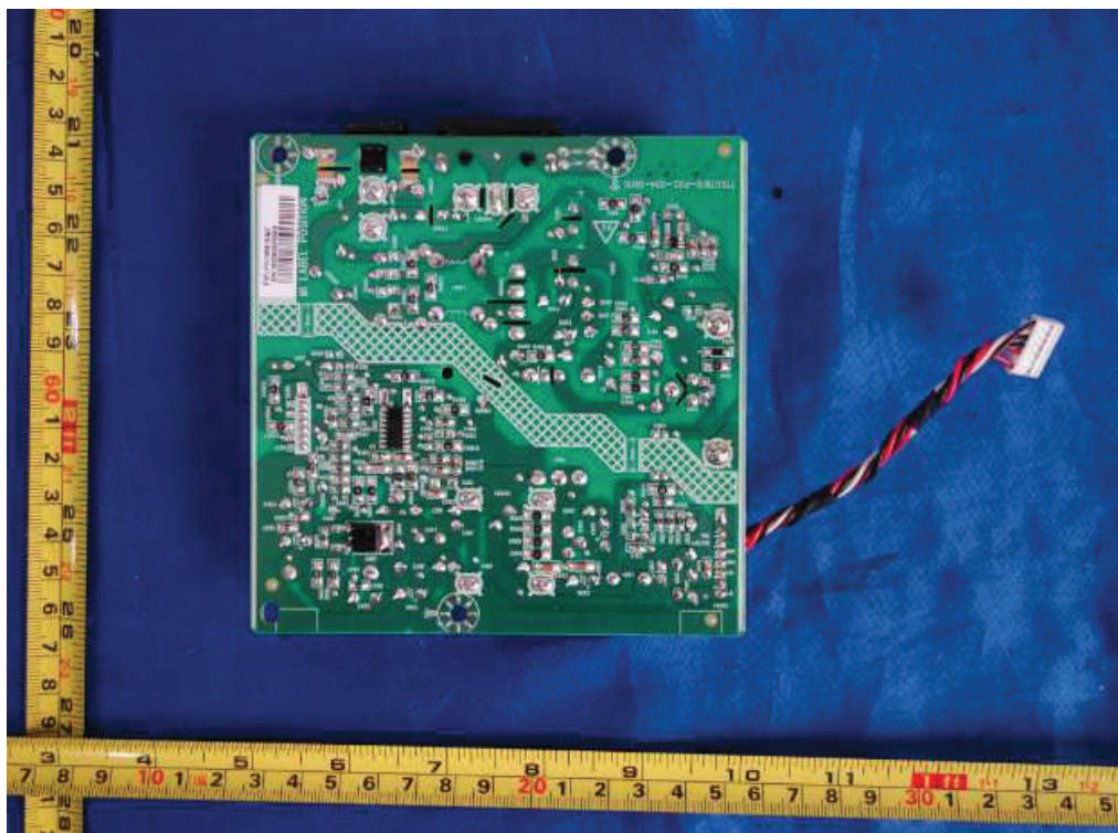
Figure 14. Power board 715G7610
