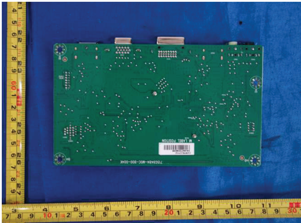
Figure 18. Main board 715G9484
