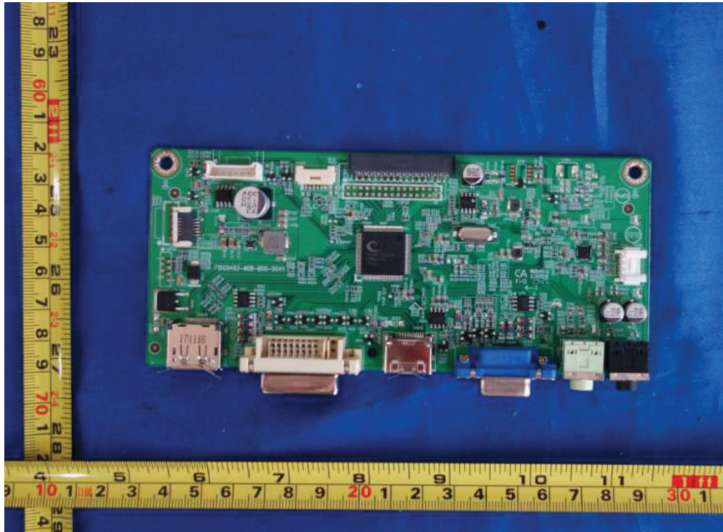
Figure 15. Main board 715G9483
