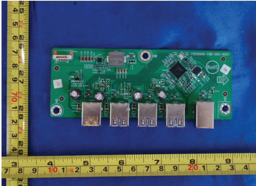
Figure 19. USB board 715G9509
