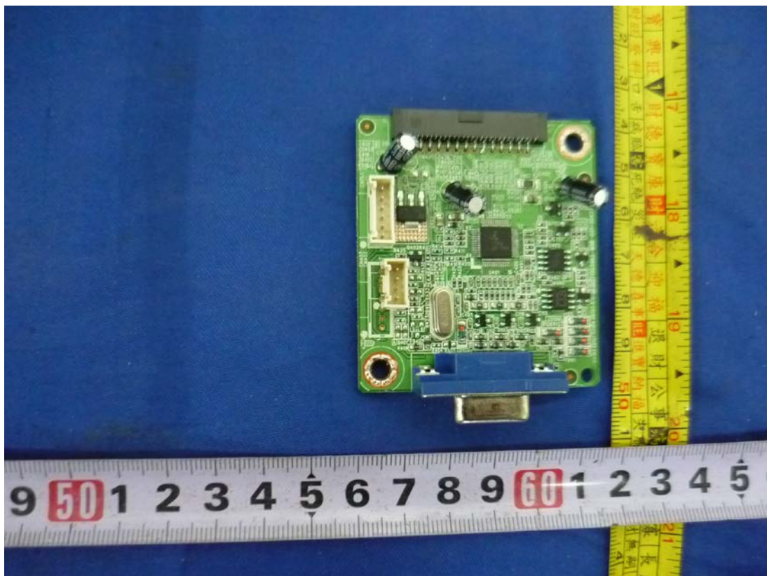
Figure 14. Main board 715G5965
