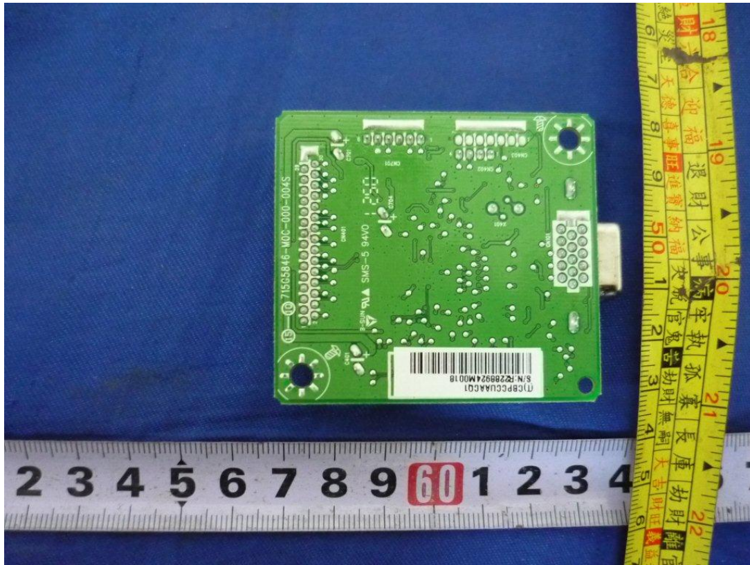
Figure 17. Main board 715G5846
