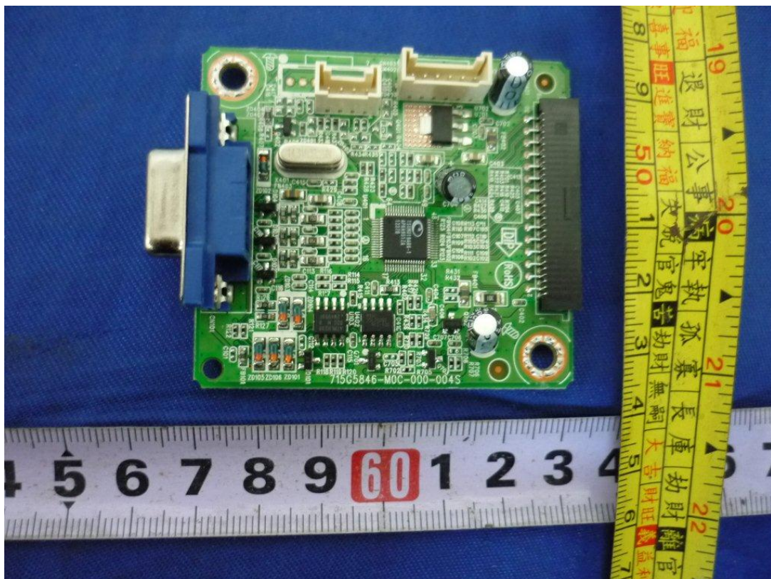
Figure 16. Main board 715G5846
