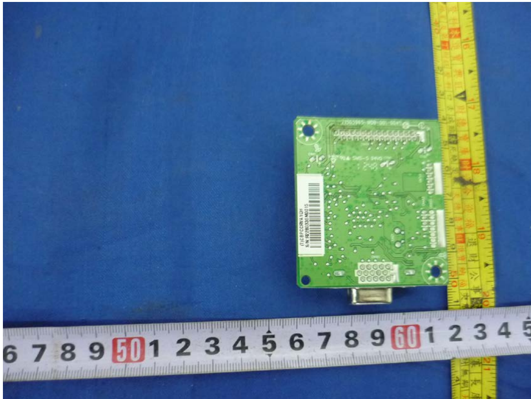
Figure 15. Main board 715G5965
