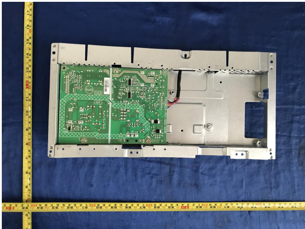
Figure 12. Internal view
