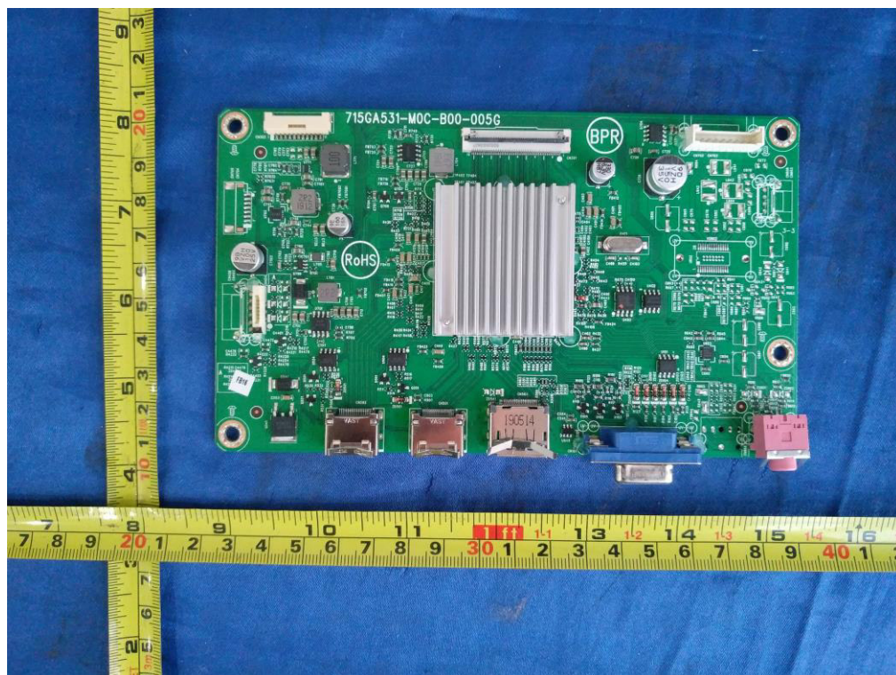
Figure 16. Main board 715GA531
