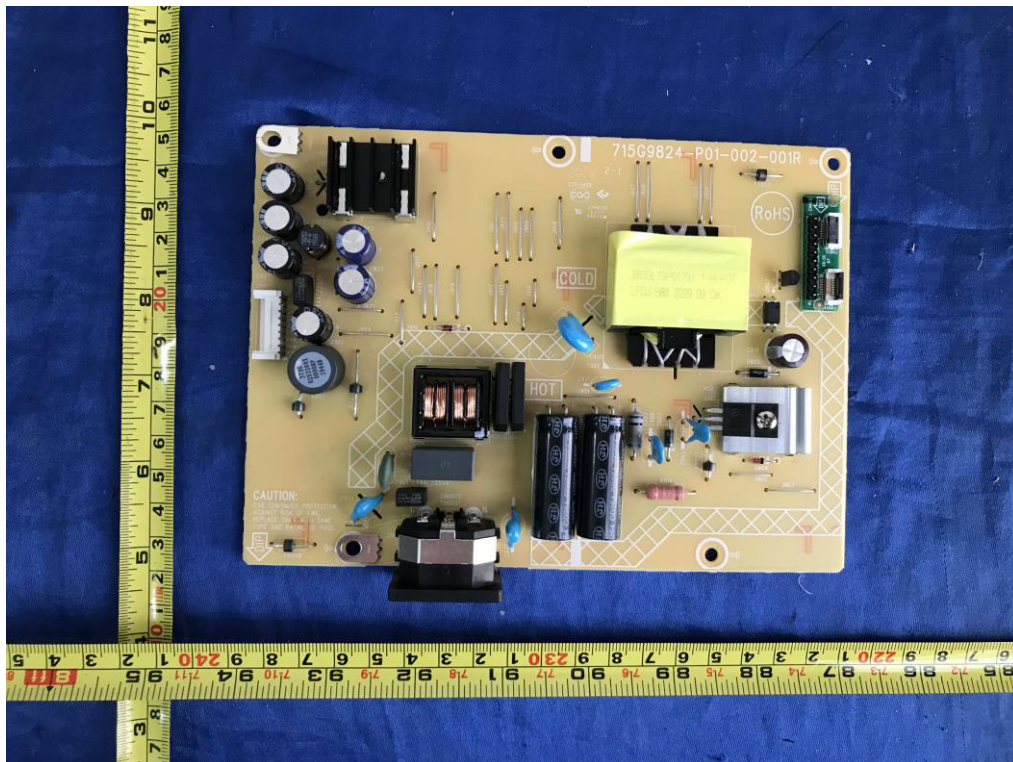
Figure 14. Power board 715G9824
