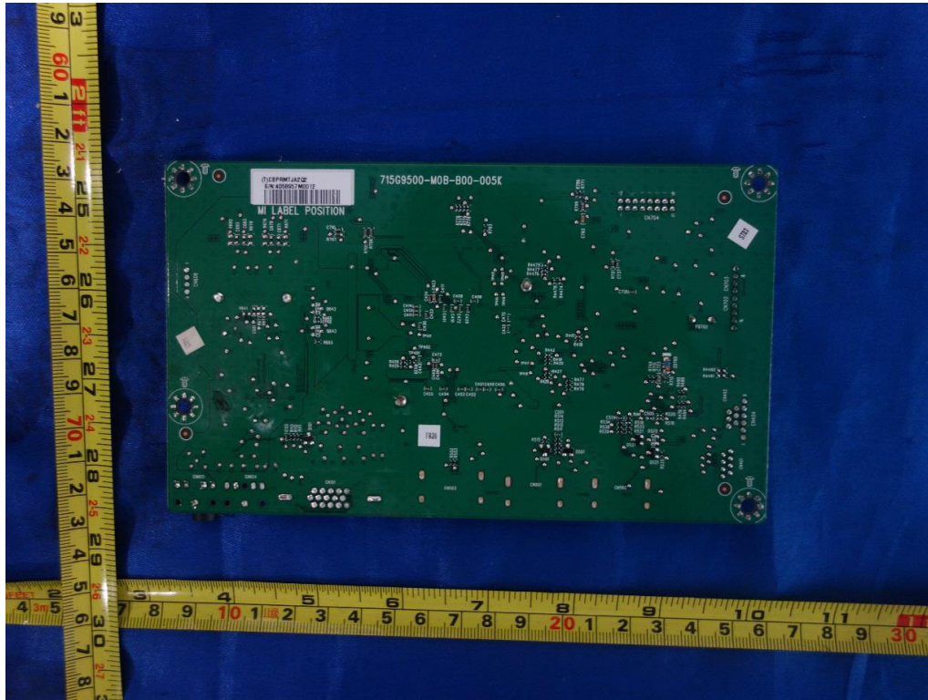
Figure 21. Main board 715G9500
