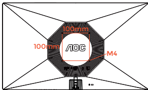
Specification of wall hanger screws: M4*(9+X)mm (X=Thickness of Wall mount bracket)
