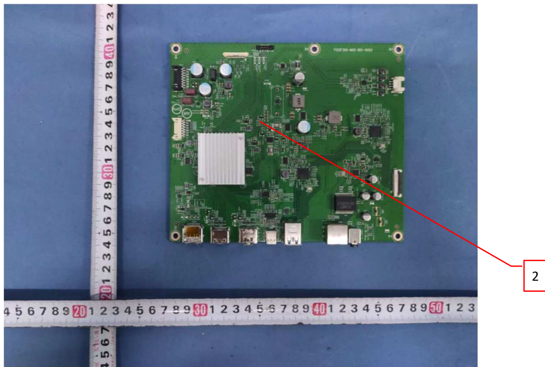
Photo 3 - Main Board (TPV/ 715GF369)
