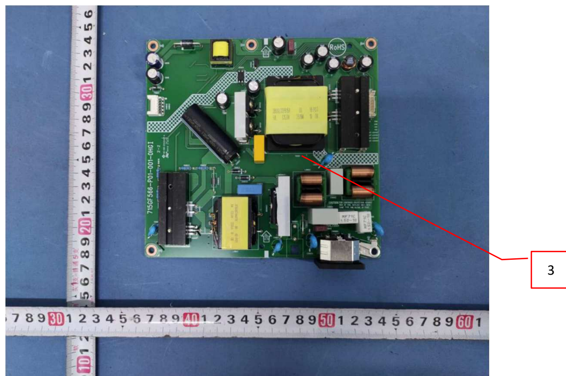
Photo 4 - Power Board (TPV/ 715GF566)
