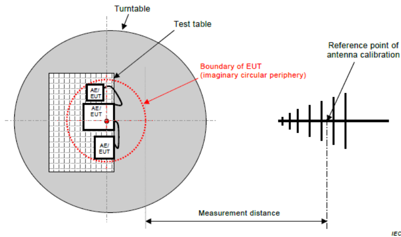
Figure C.1 – Measurement distance
