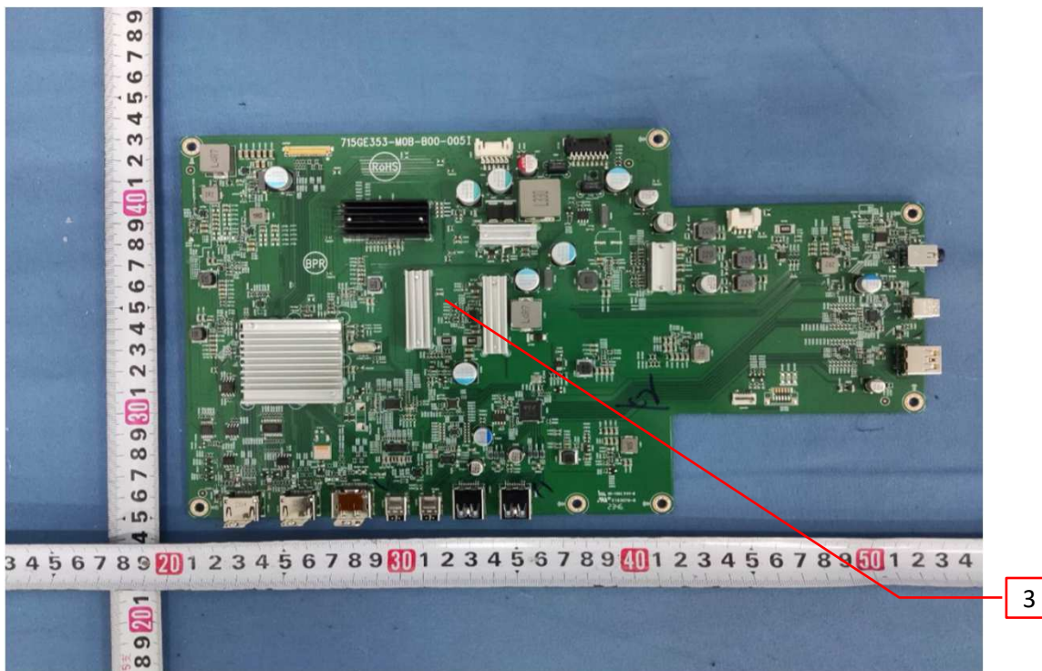
Photo 4 - Main Board (TPV/L&T/ 715GE353)
