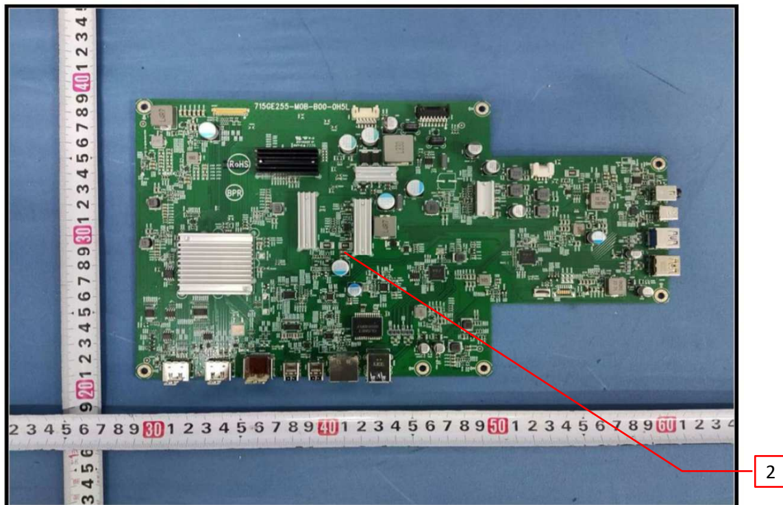
Photo 3 - Main Board (TPV/L&T/ 715GE255)
