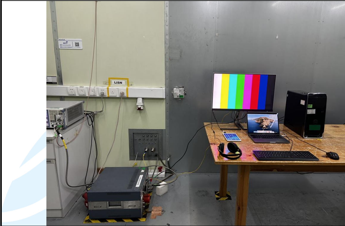
Conducted Emission (AC port) Test Setup
