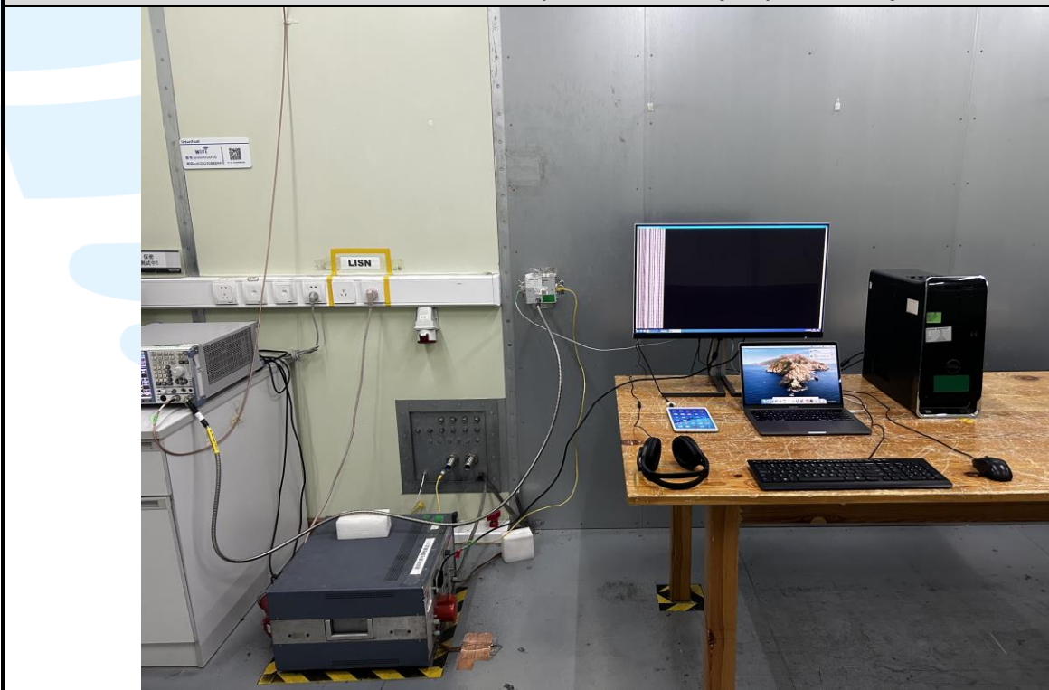
Conducted Emission (Wired network port) Test Setup
