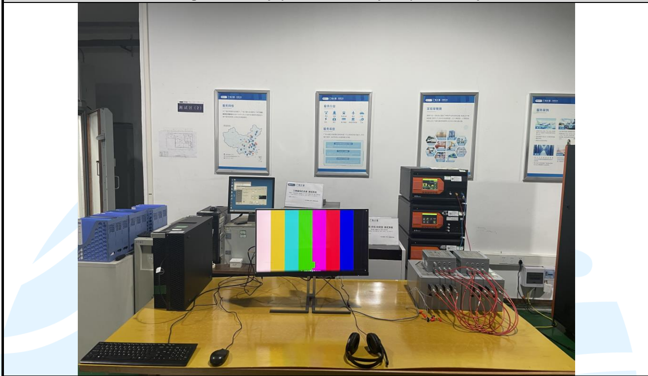
Surge Test Setup (Wired network ports) Test Setup
