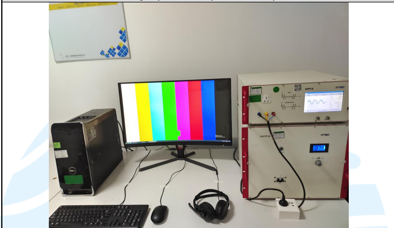
Voltage dips and interruptions Test Setup
