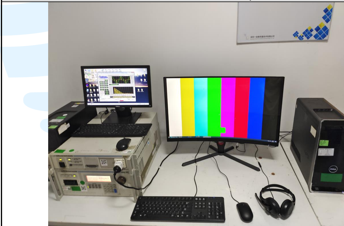
Harmonic & Flicker Test Setup
