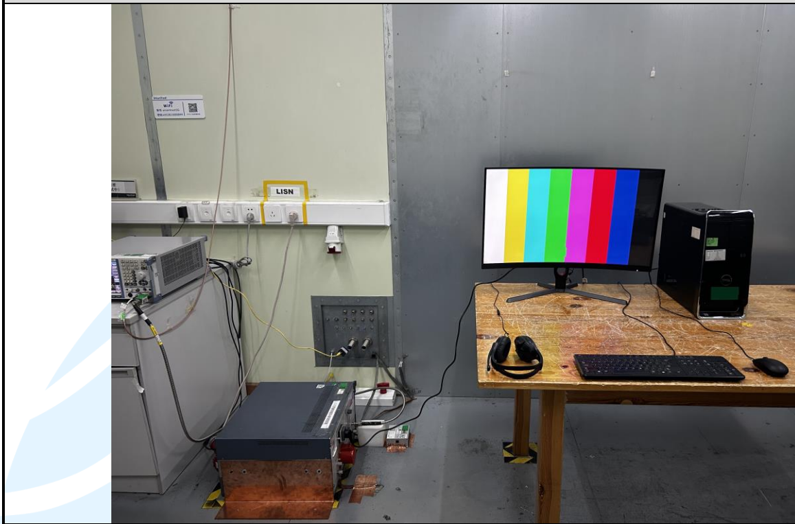
Conducted Emission (AC port) Test Setup
