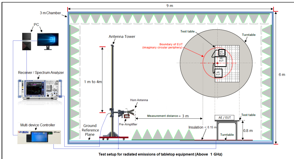
Figure 2. Above 1 GHz
