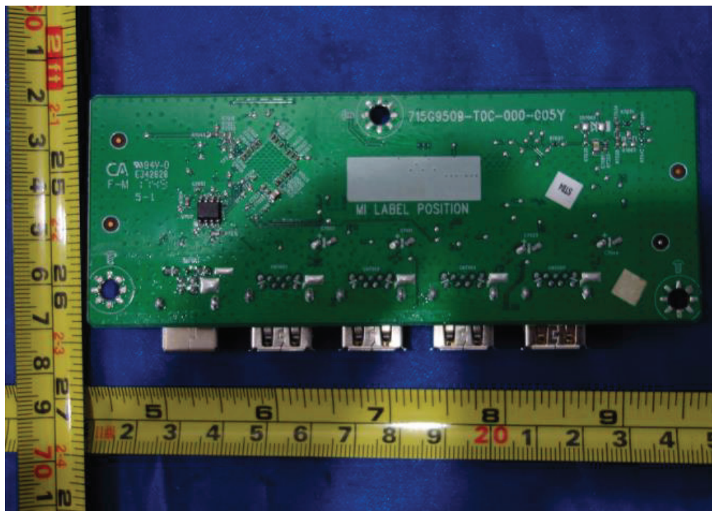
Figure 40. USB board 715G9509
