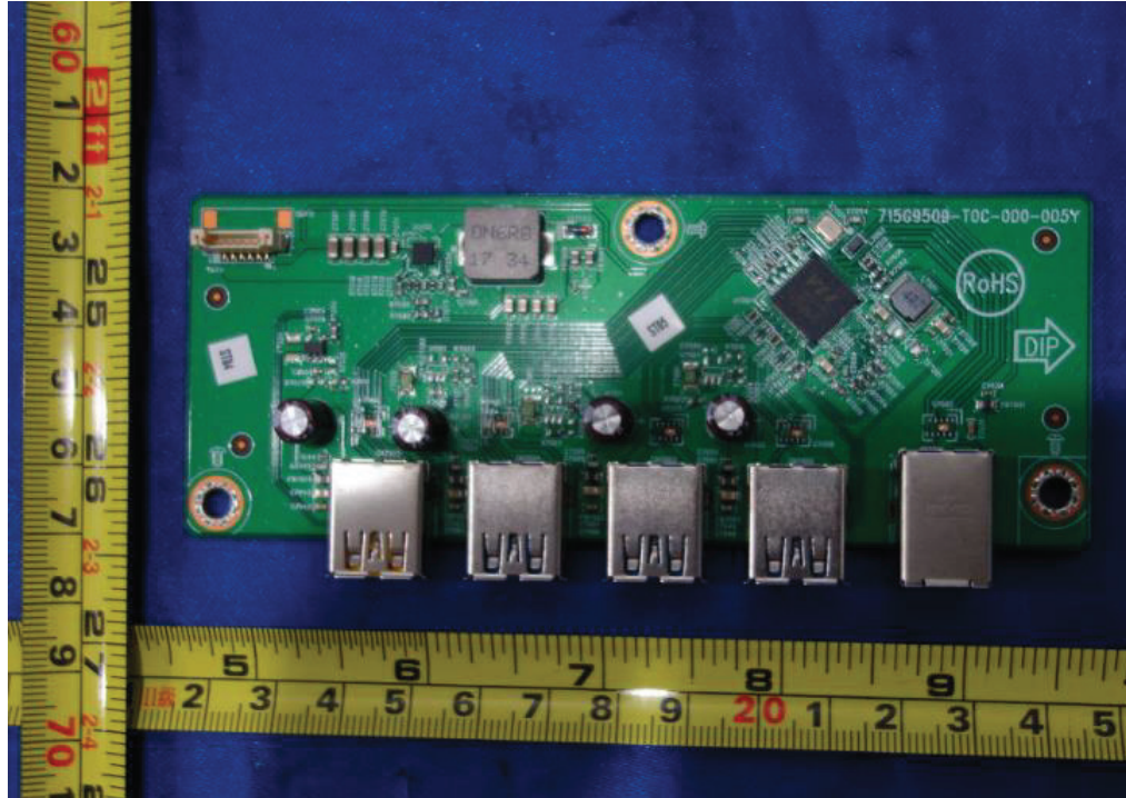
Figure 39. USB board 715G9509
