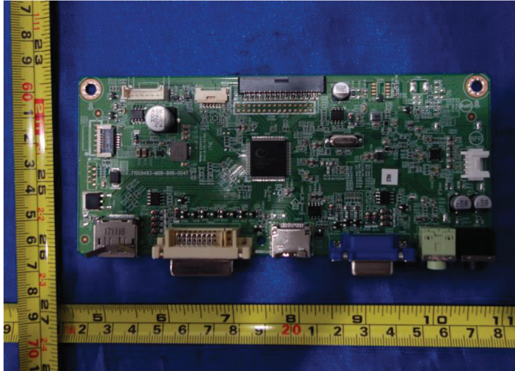
Figure 37. Main board 715G9483
