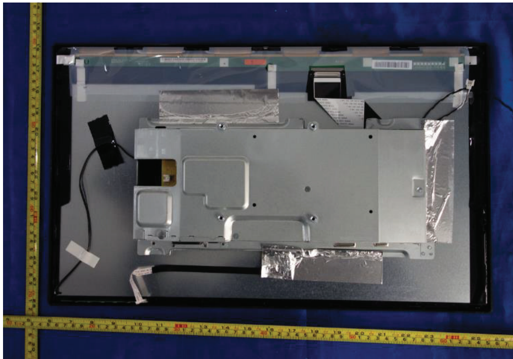
Figure 12. Metal enclosure type B with power board 715G7300 and main board 715G9496
