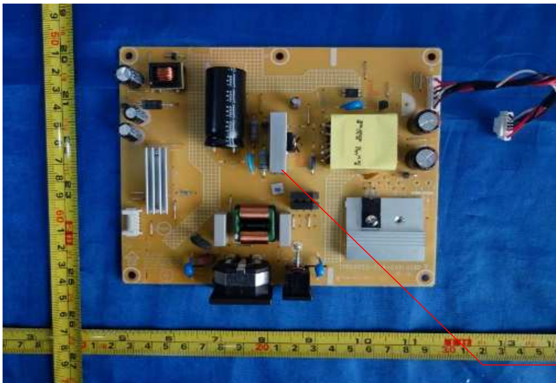
Photo 4 - Power board (TPV / 715G8852)
